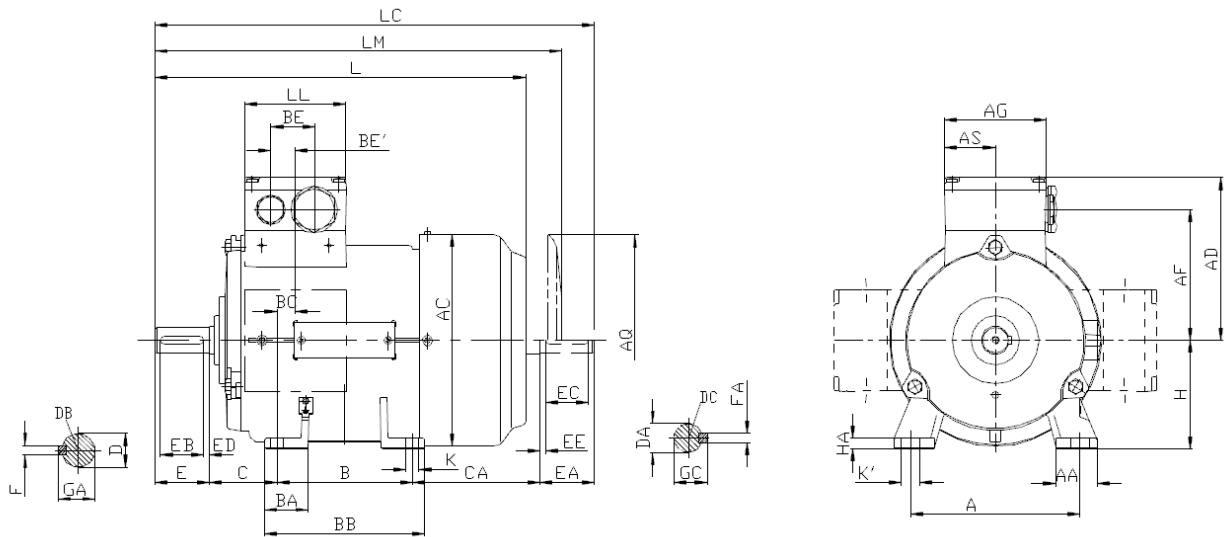
Flanschbaufornen flange type of construction
